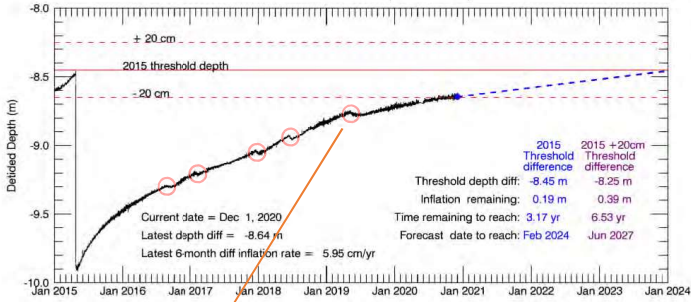
Long-term inflation of central caldera
